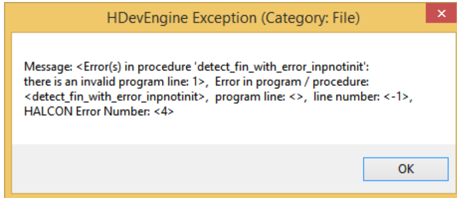
Figure 23.6: Content of the exception if an input parameter was not initialized.
