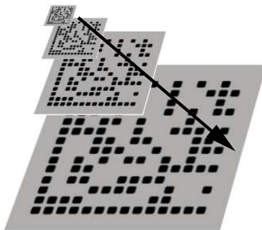
Figure 3.12: Pyramid levels.
