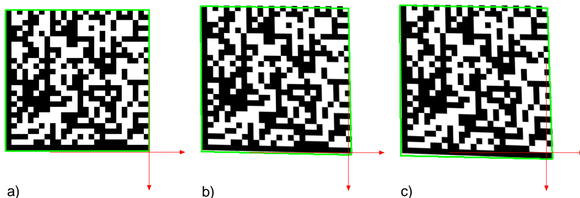
Figure 6.6: Quality grades for grid non-uniformity: (a) 4, (b) 2, and (c) 0.
